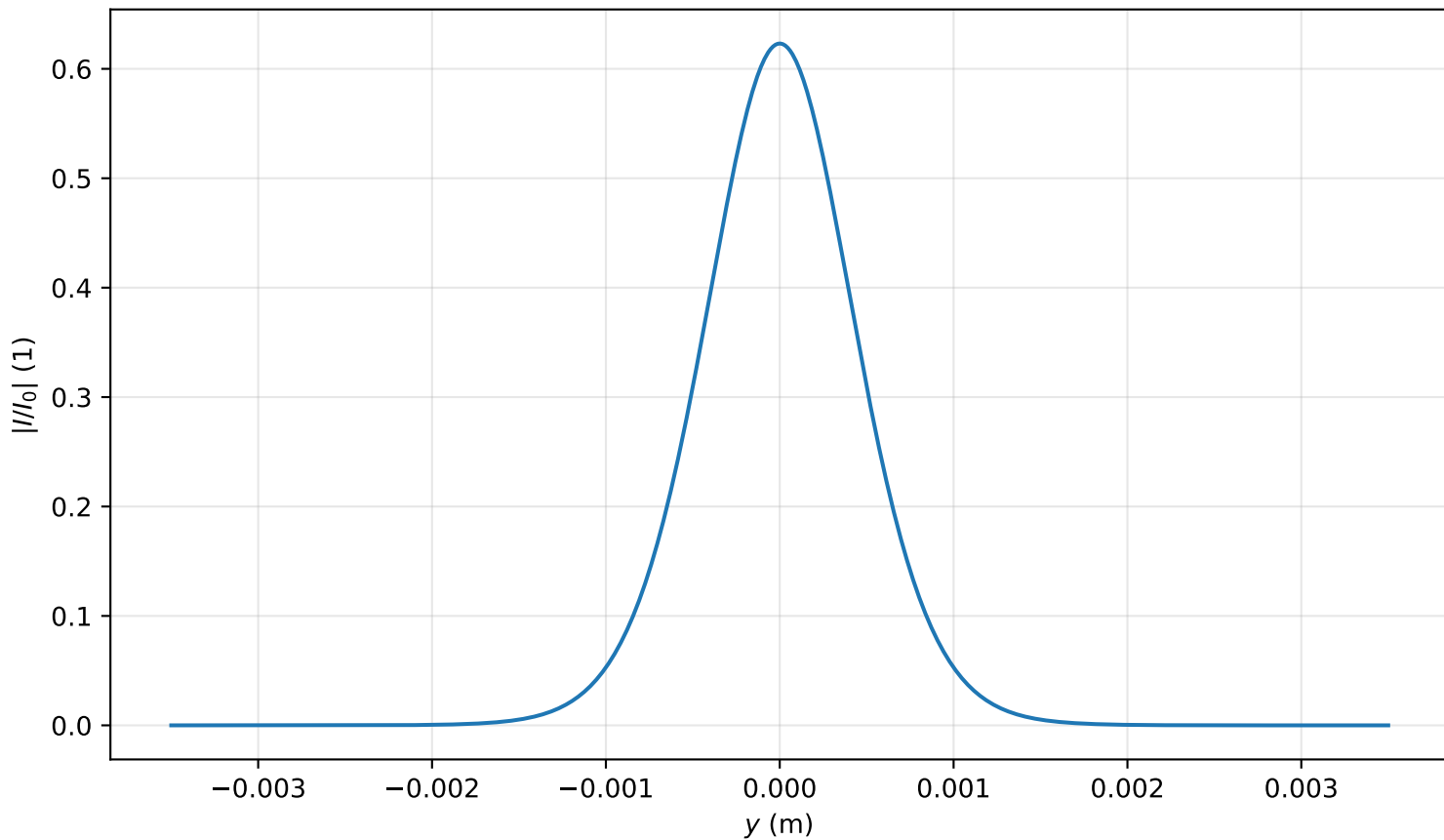
Intensity profile I(x=0, y, z=2.388)/I_0 , P_{in}=0.4P_{cr} , artificial time
